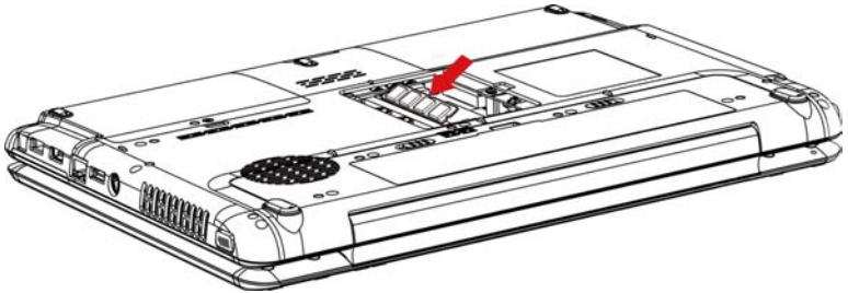
Figure 8-8 Inserting the memory module
